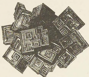
BISMUTH.
